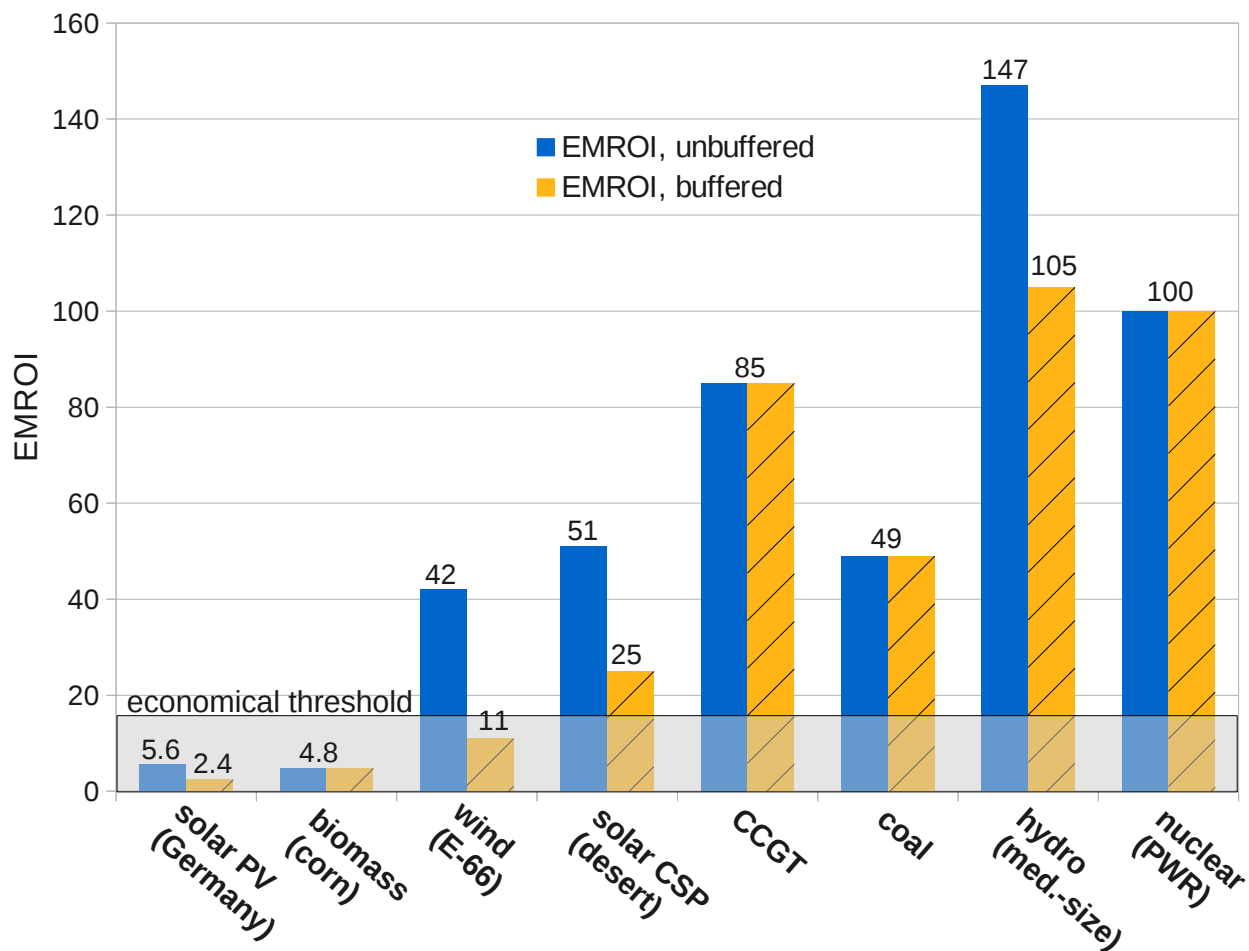
Figure 2: (Color online.) EMROIs of all energy techniques with economic "threshold" based on the current production cost ratio electricity/thermal energy of w = 3 . The weighting factor w is expected to decrease with time, approaching 1 or even lower, which makes the EMROI identical to the EROI as shown in Fig. 3.
