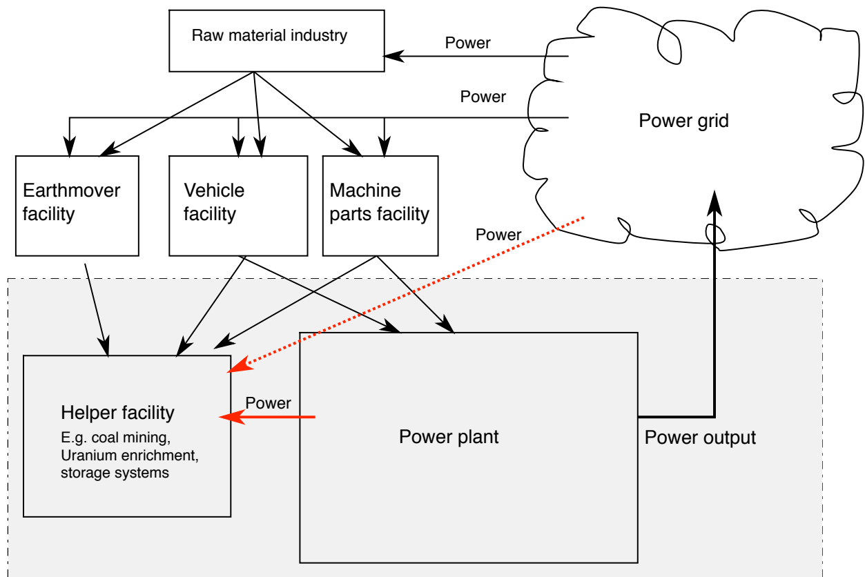
Figure 1: System borders for a typical power plant. It makes a difference if electricity for a helper facility like a coal mine is taken from the grid (dashed line) or from the power plant.
